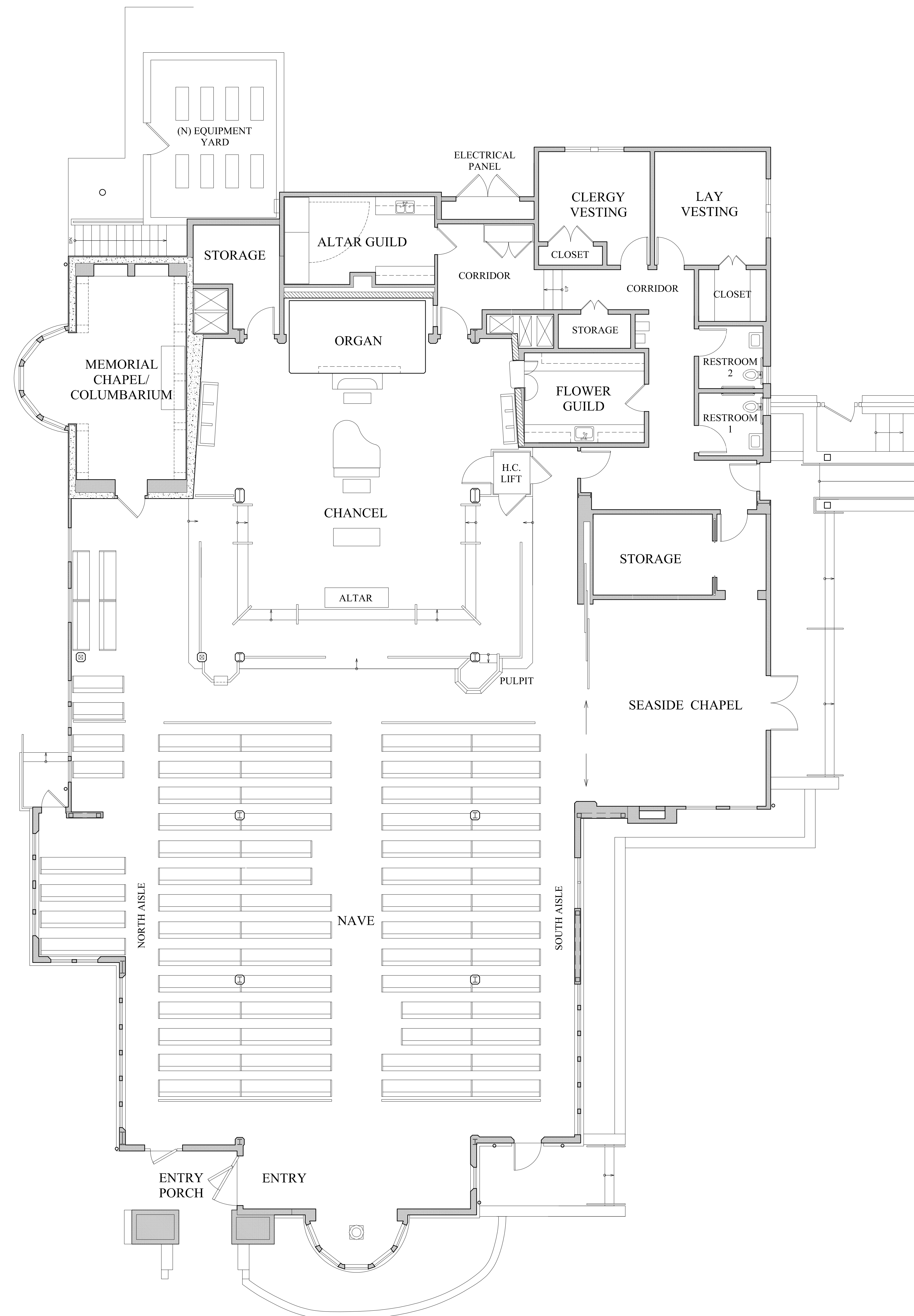
Proposed Floor Plan
