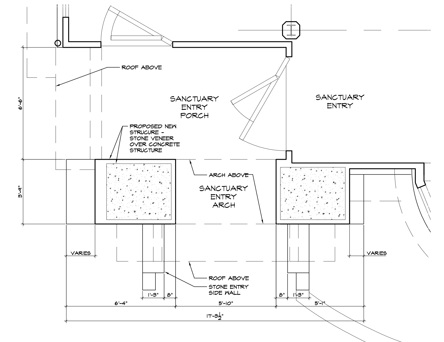
5 Architectural Plan @ Bell Tower SCALE : 3/8" = 1'-0"
