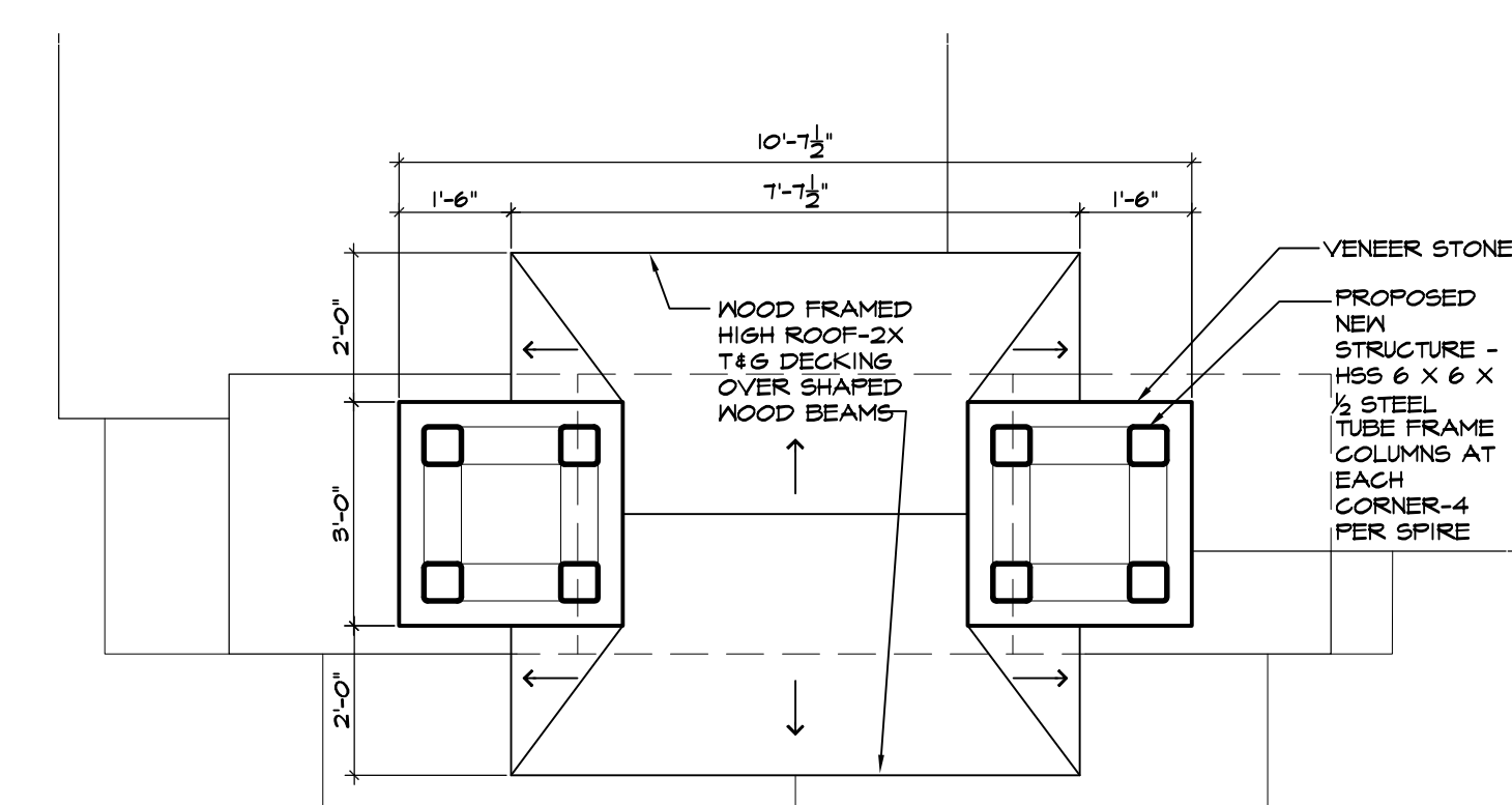
9 Architectural Plan @ Bell Tower SCALE : 3/8" = 1'-0"
