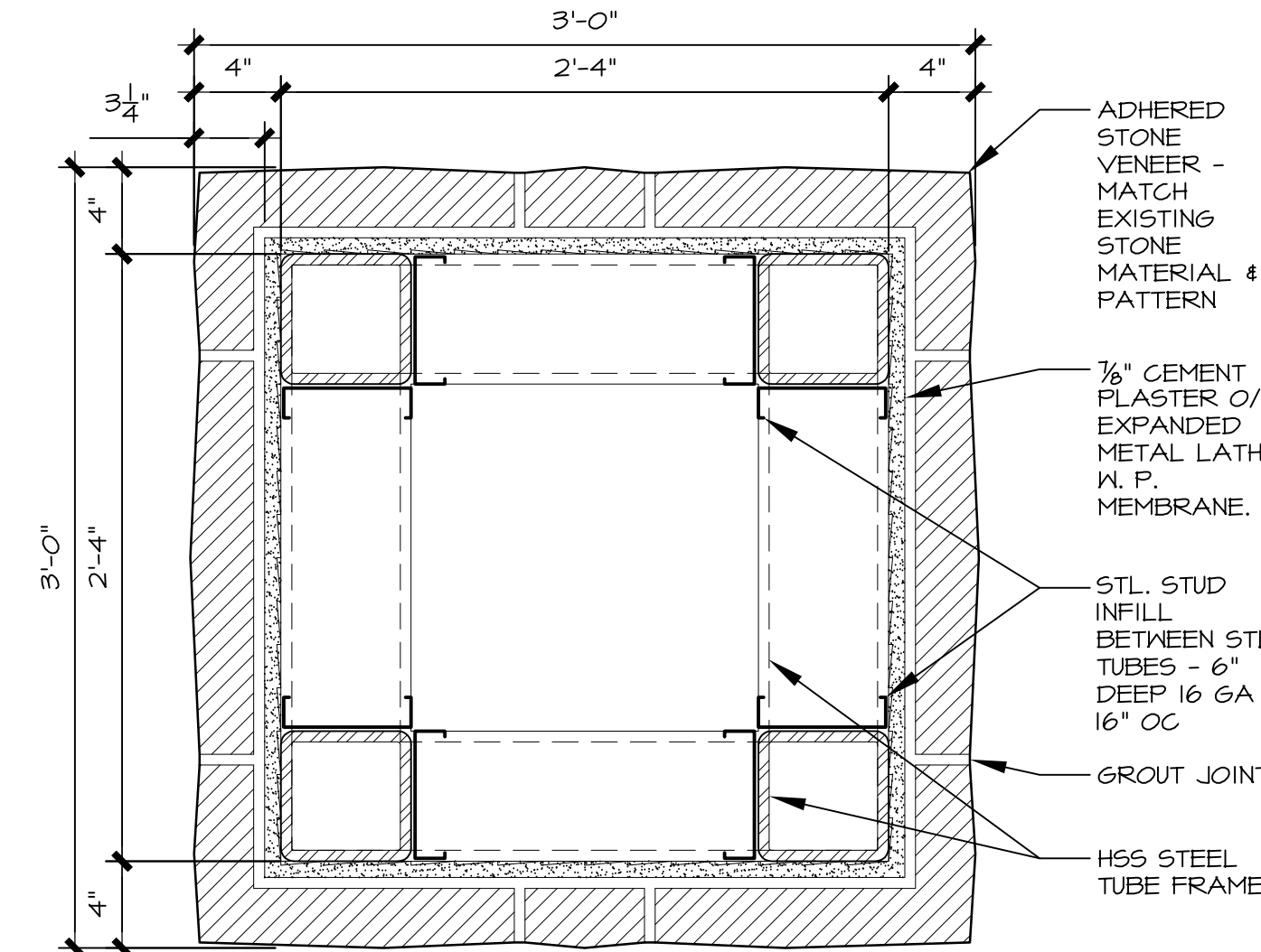
6 BELL TOWER PROPOSED SPIRE DETAIL SCALE : 1 1/2" = 1'-0"
